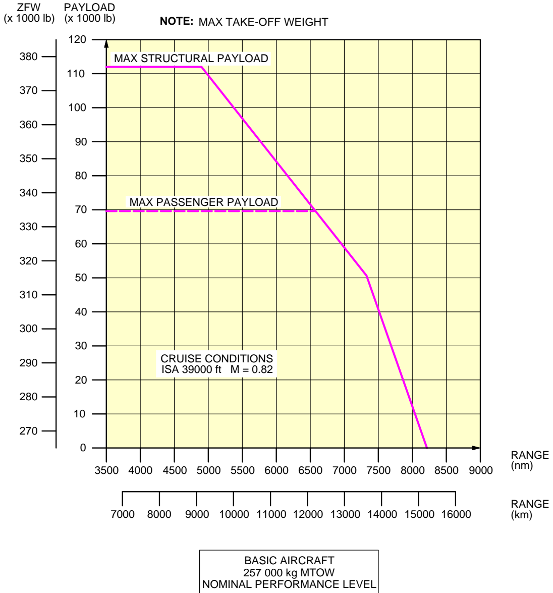
Payload / Range - ISA Conditions CFM56-5C4 engine FIGURE-3-2-1-991-015-A01
