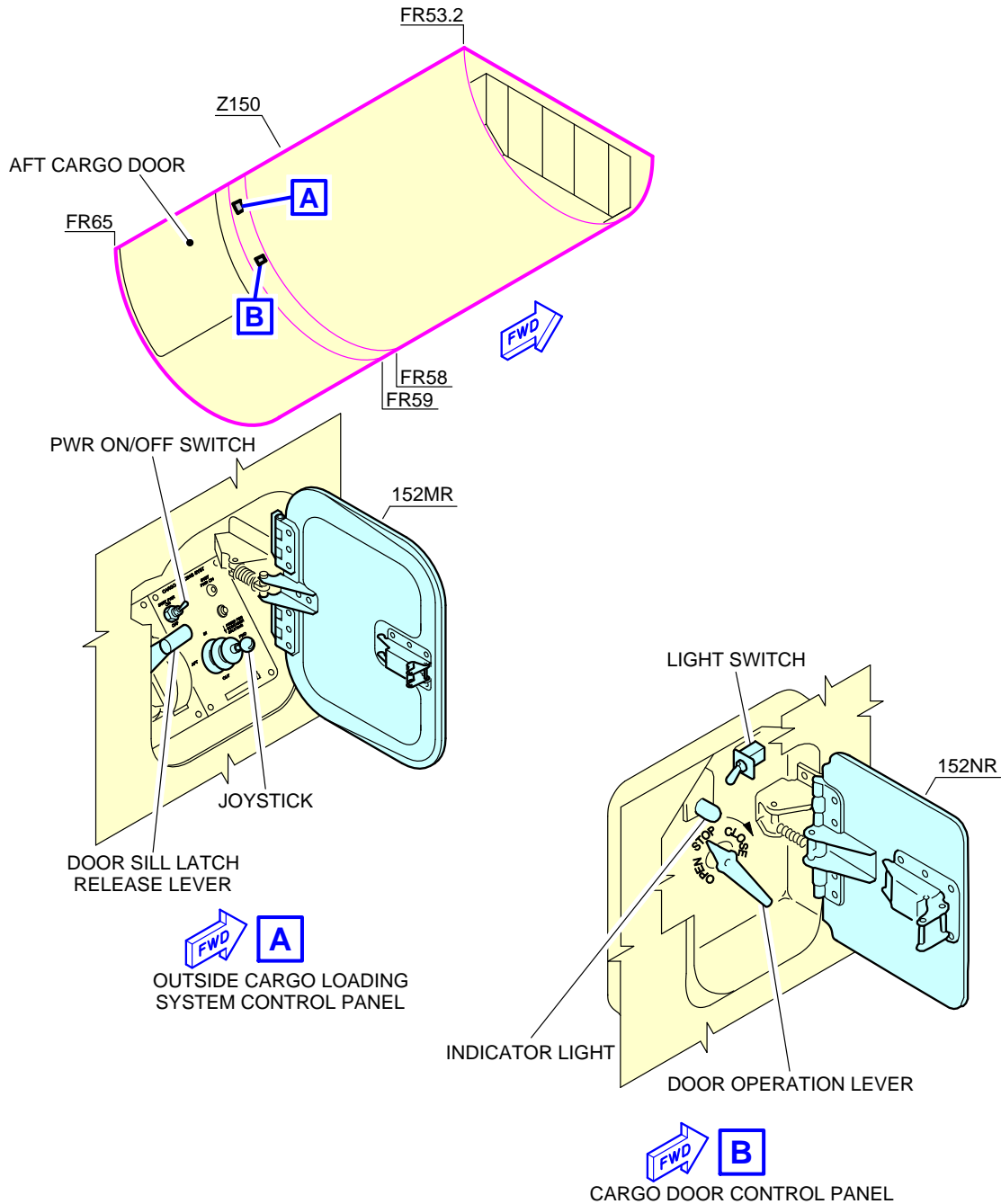
Aft Cargo Control Panels FIGURE-5-4-11-991-005-A01
