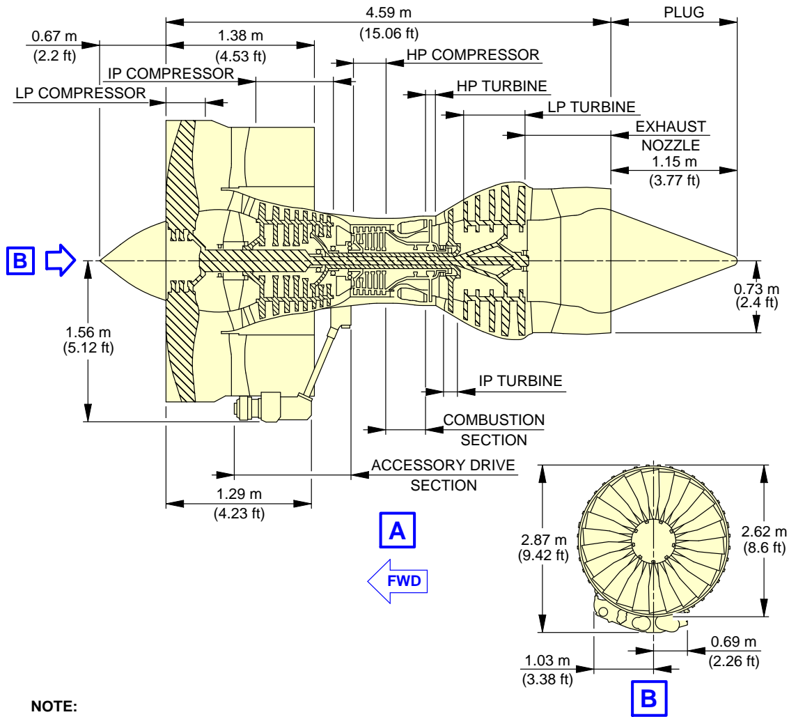
Engine and Nacelle Engine Dimensions - TRENT 500 FIGURE-2-12-0-991-021-A01
