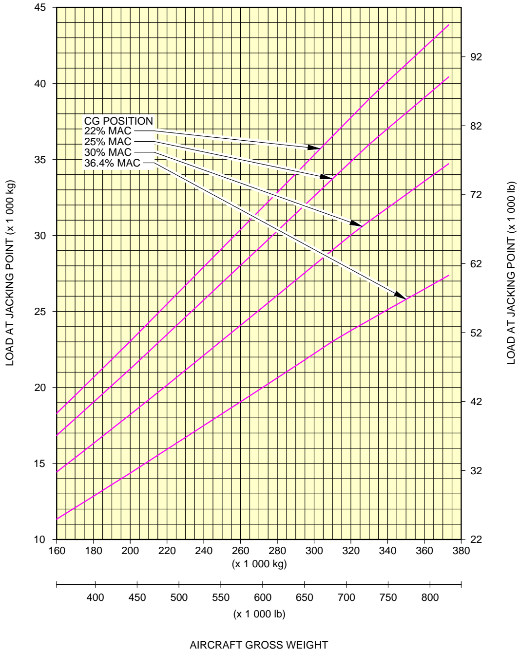
Jacking of the Landing Gear NLG Jacking Point Loads - (WV 001) FIGURE-2-14-1-991-020-A01
