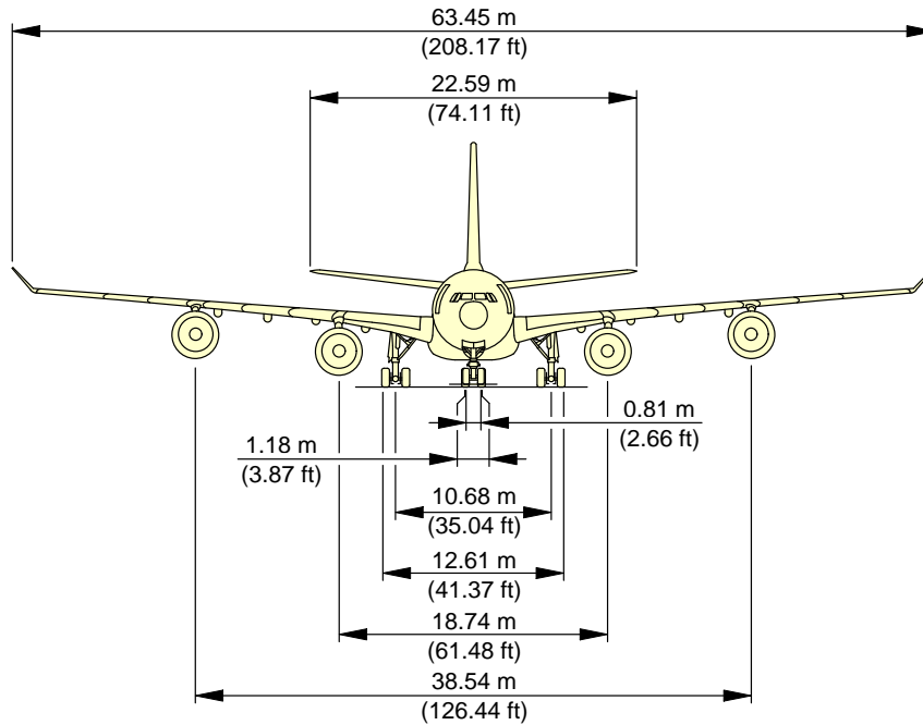
General Aircraft Dimensions (Sheet 1 of 2) FIGURE-2-2-0-991-009-A01
