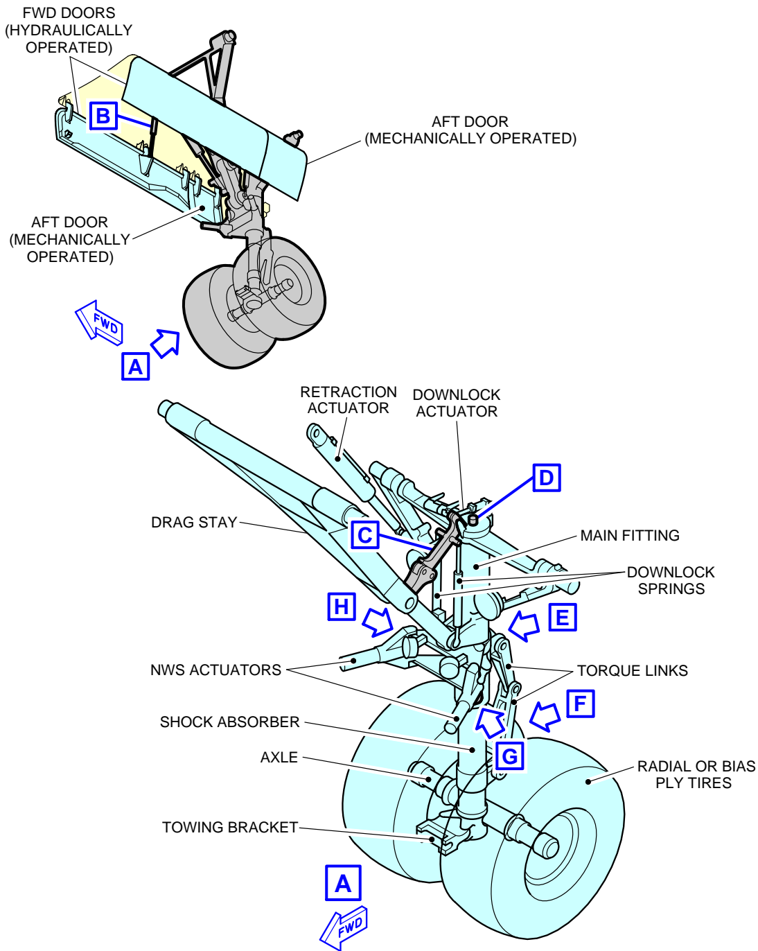
Nose Landing Gear General (Sheet 1 of 4) FIGURE-2-9-0-991-014-A01
