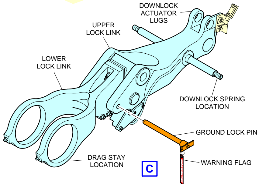
Nose Landing Gear Safety Devices (Sheet 2 of 4) FIGURE-2-9-0-991-014-A01
