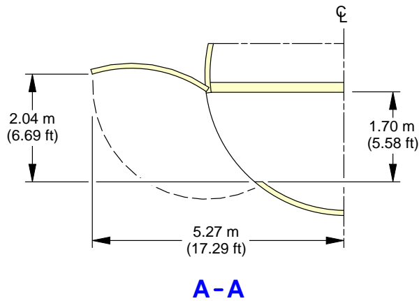
Door Clearances Forward Cargo Compartment Door FIGURE-2-7-0-991-047-A01
