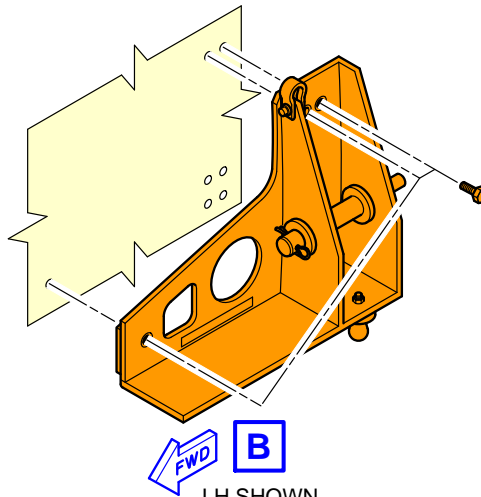
Support of Aircraft Location of Auxiliary Jacking Points (Sheet 2 of 2) FIGURE-2-14-2-991-003-A01
