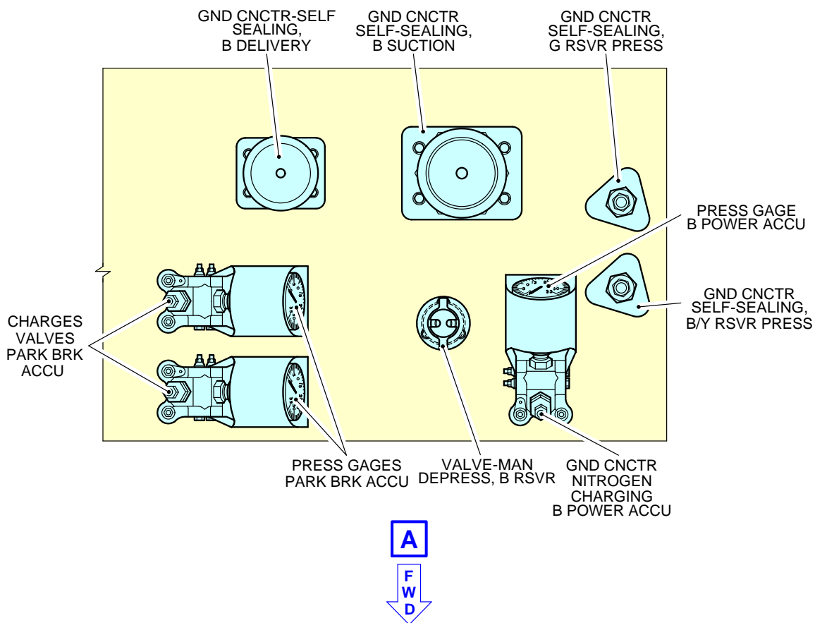
Ground Service Connections Blue System Ground Service Panel FIGURE-5-4-3-991-008-A01
