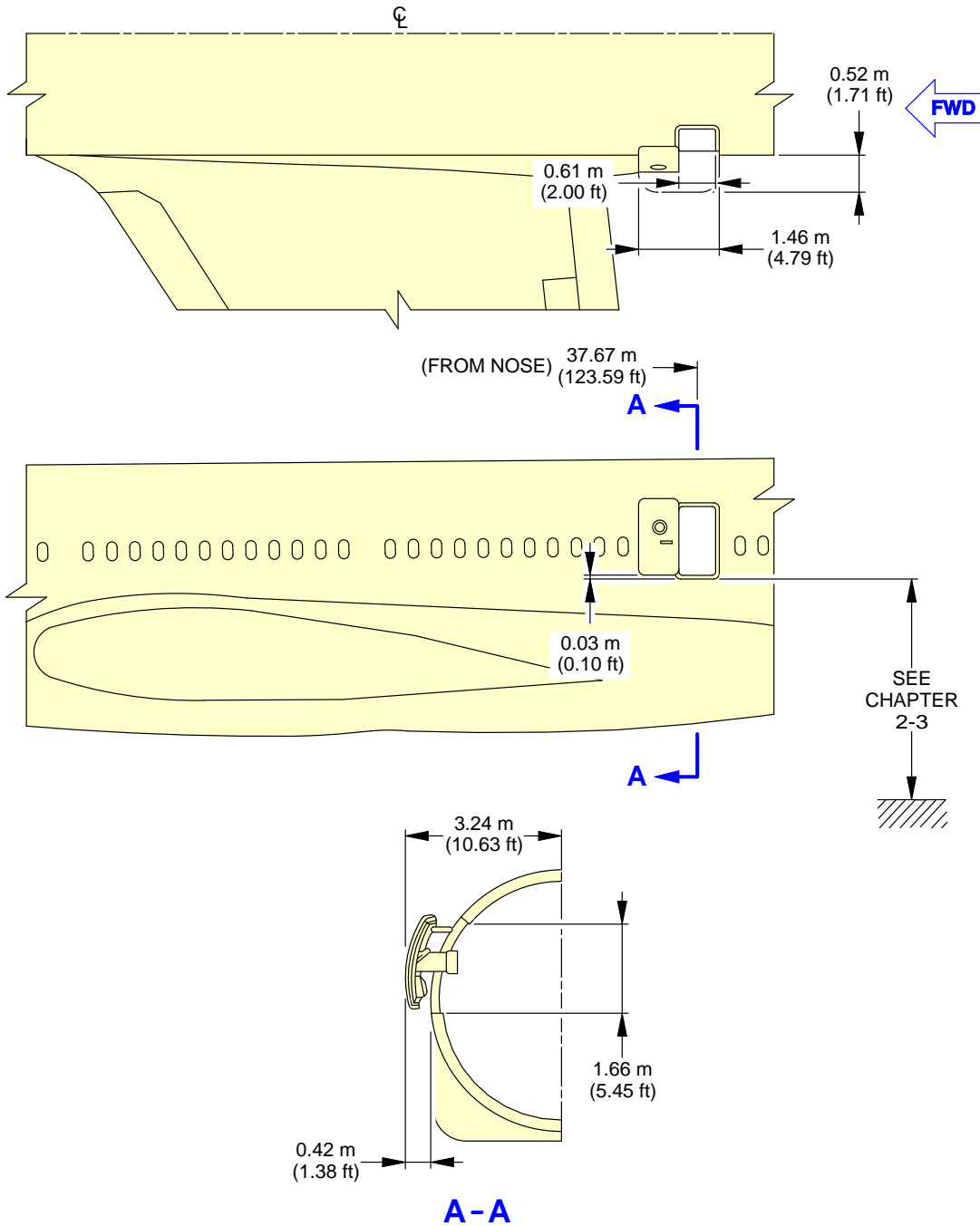
Door Clearances Emergency Exits FIGURE-2-7-0-991-044-A01
