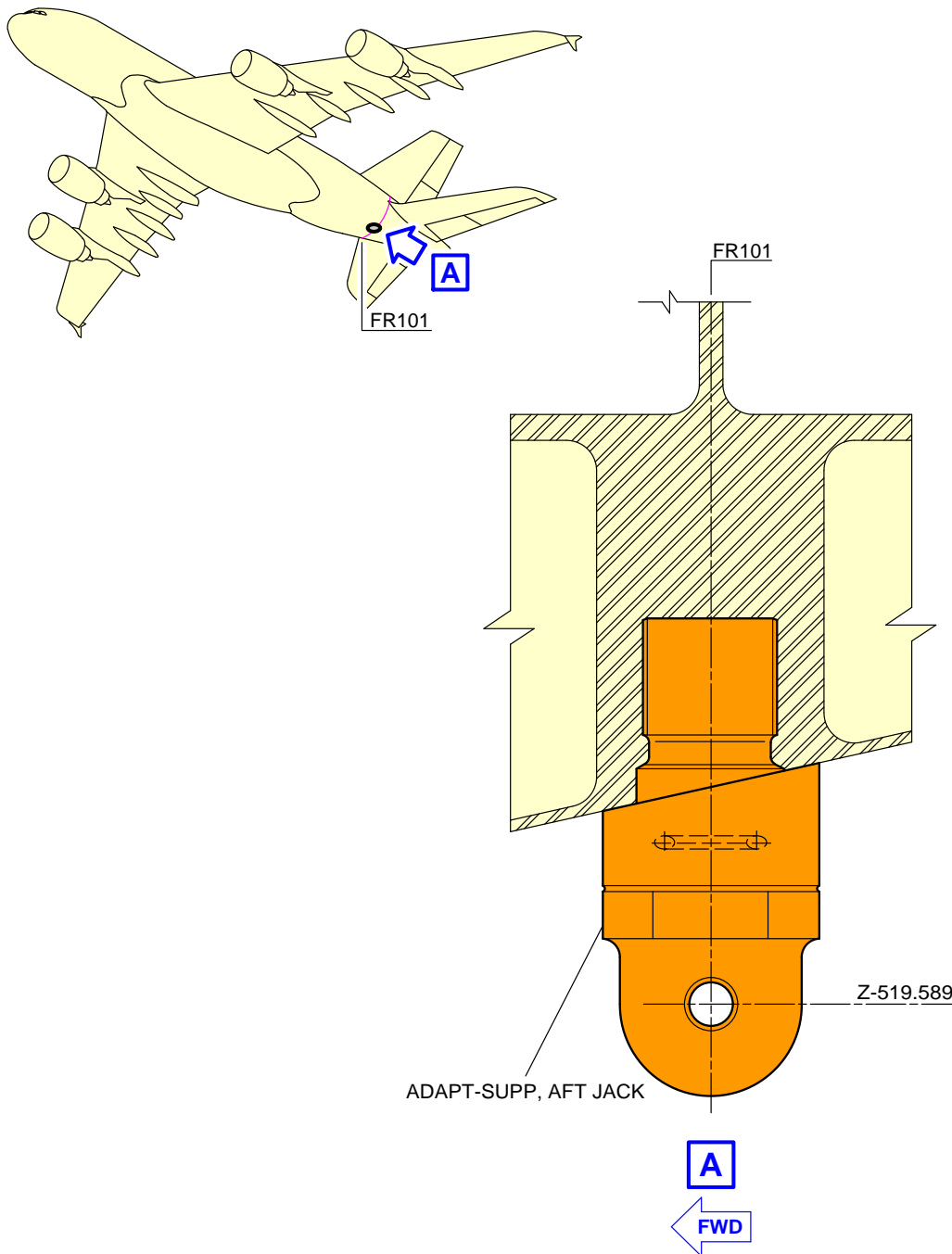
Jacking for Maintenance Auxiliary Jacking Point - Safety Stay FIGURE-2-14-0-991-011-A01
