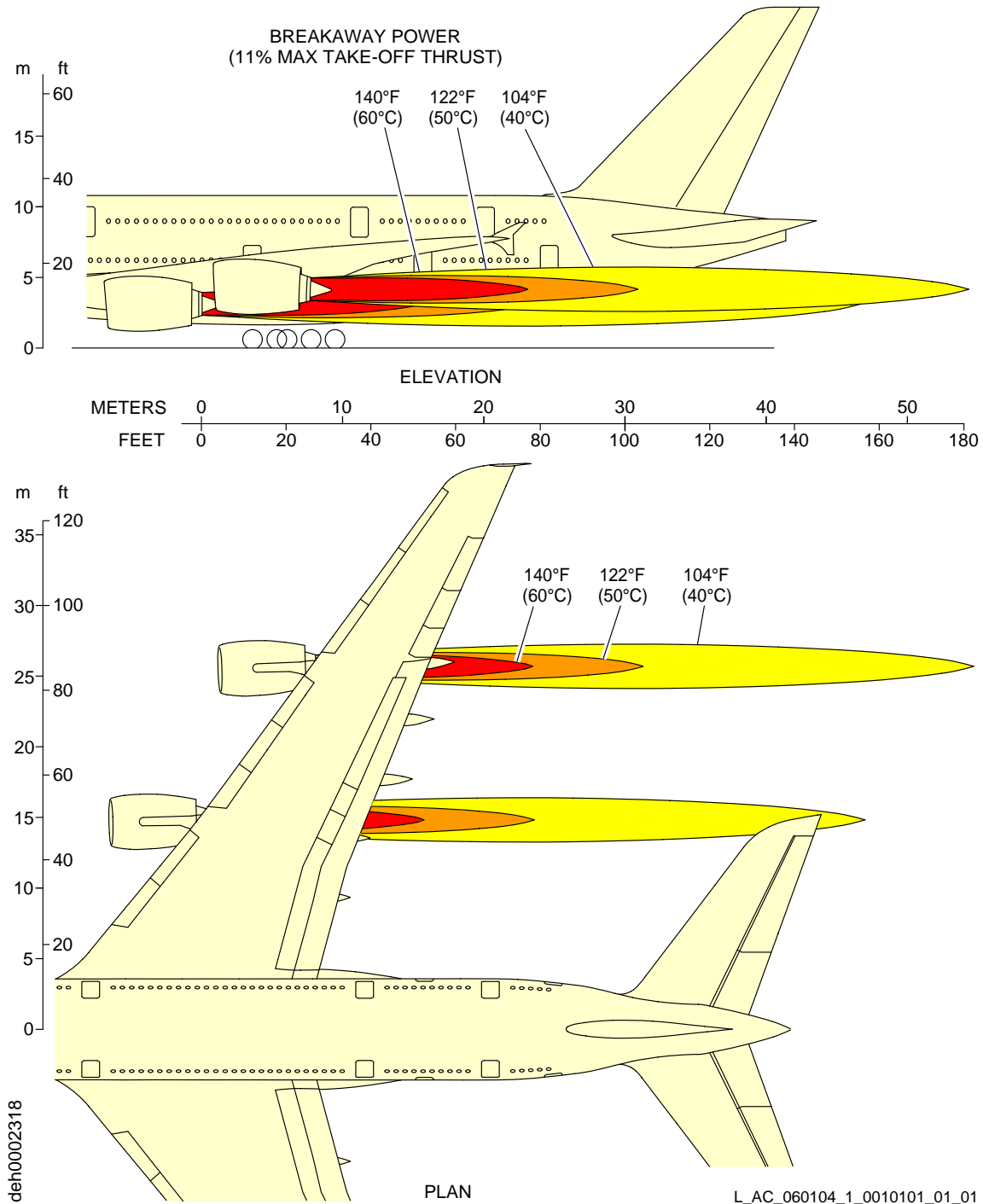
Engine Exhaust Temperatures Breakaway Power - TRENT 900 Engines FIGURE-6-1-4-991-001-A01
