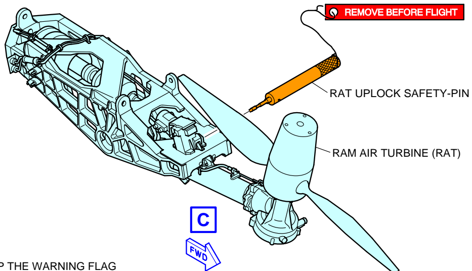
Ground Service Connections Ram Air Turbine Retracted FIGURE-5-4-4-991-005-A01
